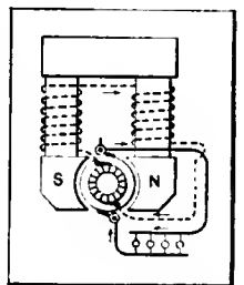
Fig. 13—Diagram of a separate-circuit, self-exciting generator
